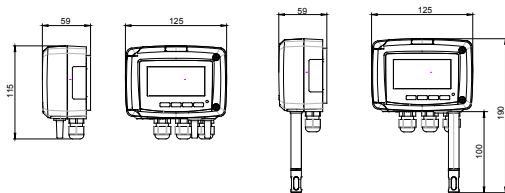
Remote model
