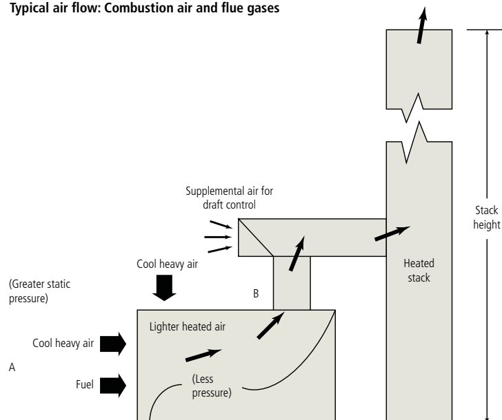
Typical air flow: Combustion air and flue gases
