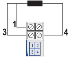
Electrical connection of the converter (Pt100 3-wire)
